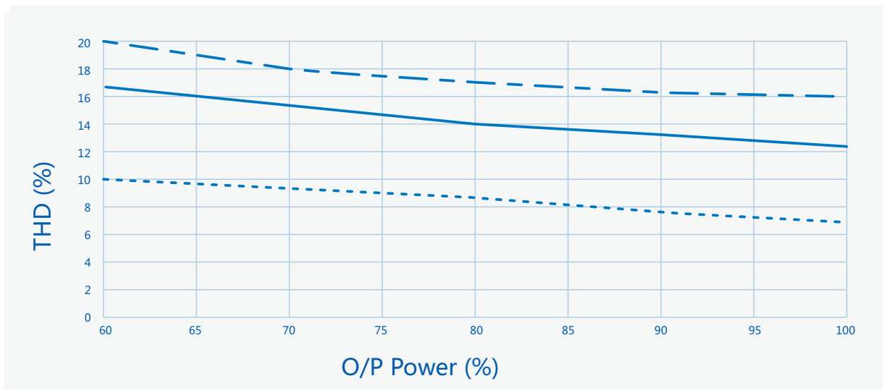
THD Vs. O/P Power
